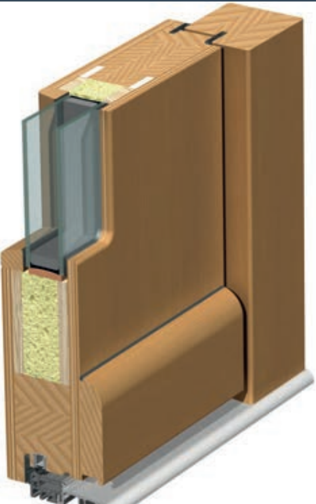
Modern Series 68mm profile U-Value 1.1 W/m²K
